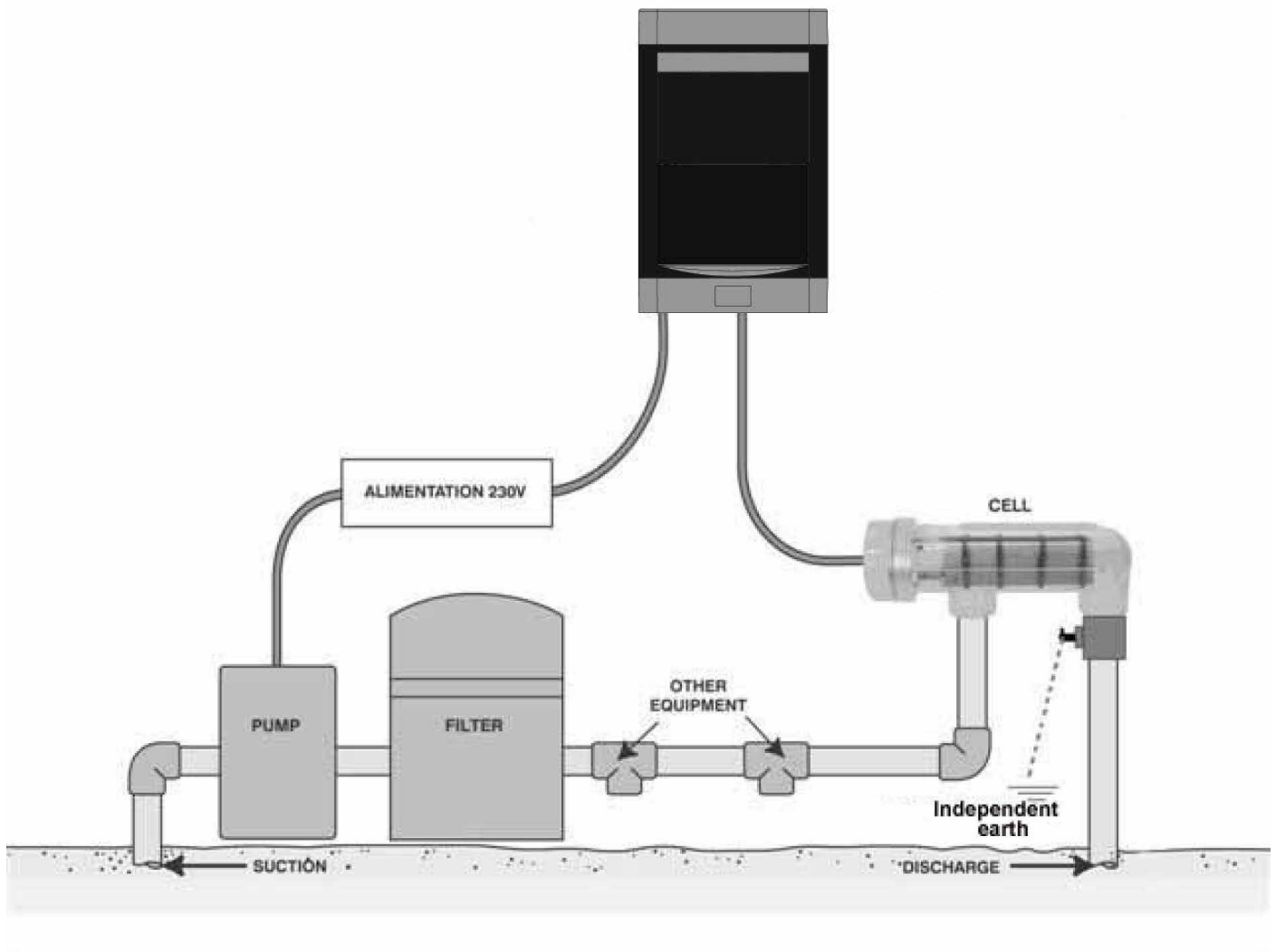
MPS50CE Cell
